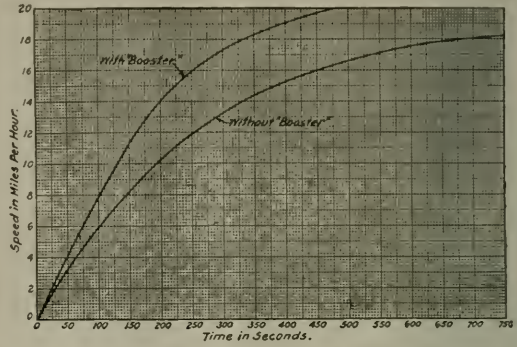
FIG. 2. ACCELERATION CURVES AND STEAM PRESSURE CURVES
